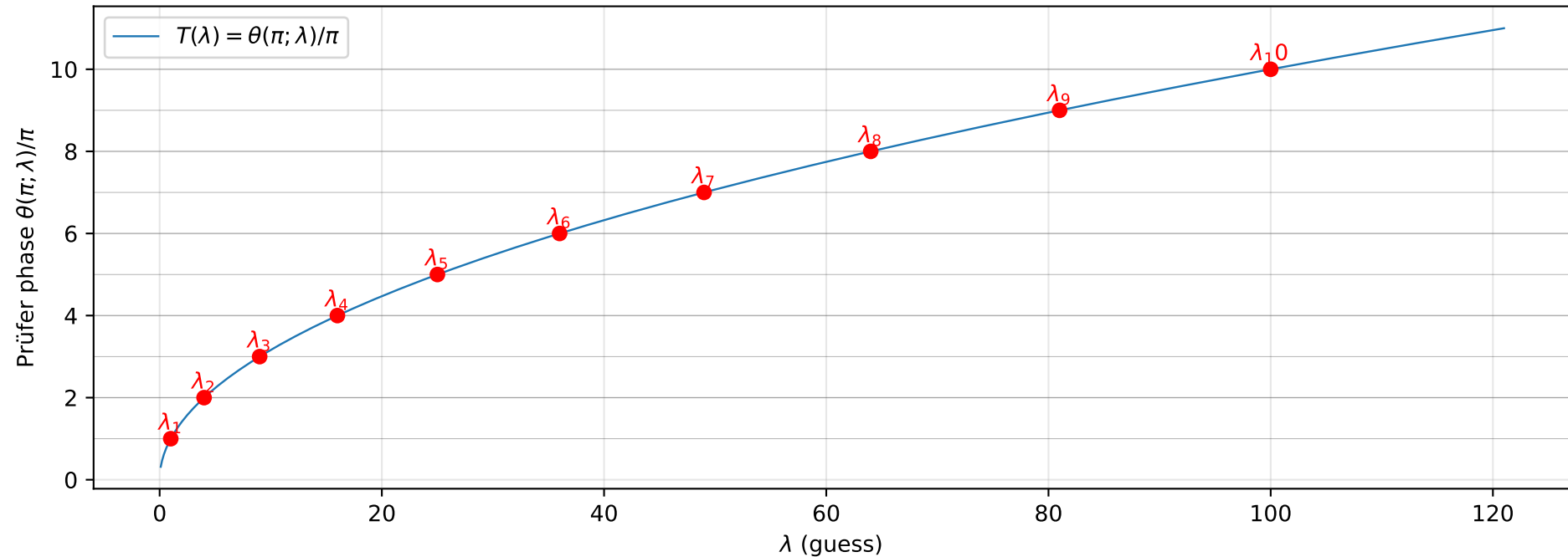
Prüfer phase sweep on graded grid (n=100, ratio=1.3) for 10 eigenvalues
